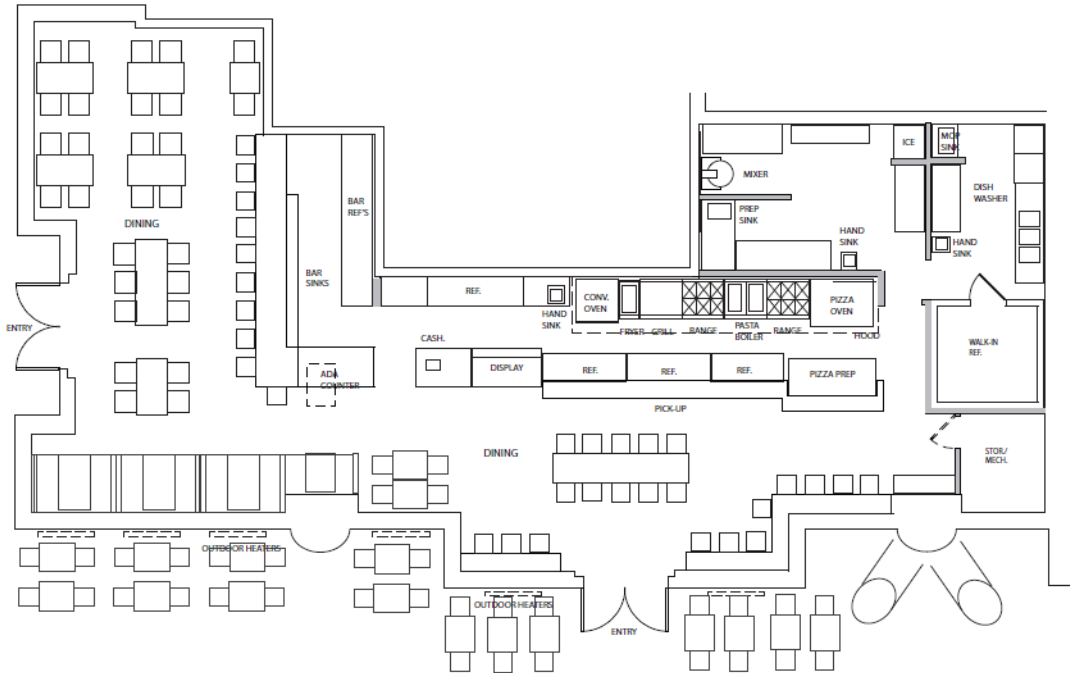
ACQUOLINA PRELIMINARY FLOOR PLAN 1/8" = 1'-0"
