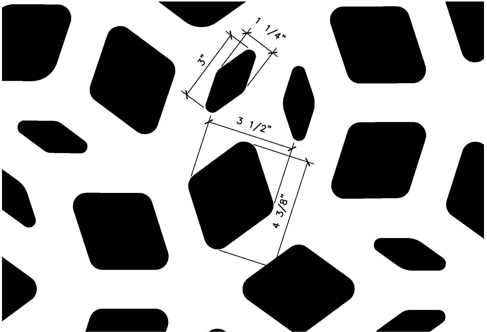
PANEL TYPE A – REVISED PERFORATION SCALE
