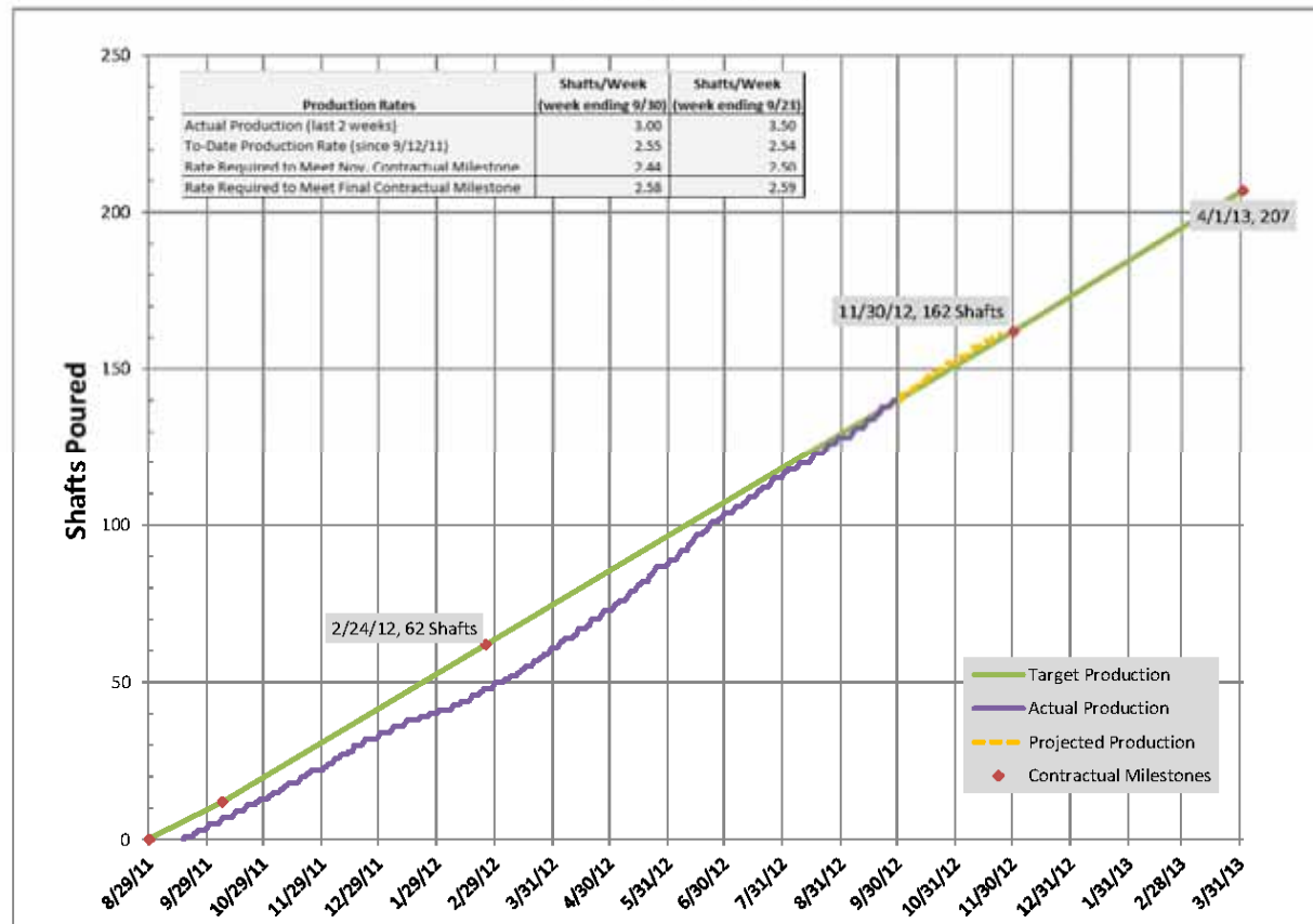
Transbay Transit Center Buttress Shaft Production
